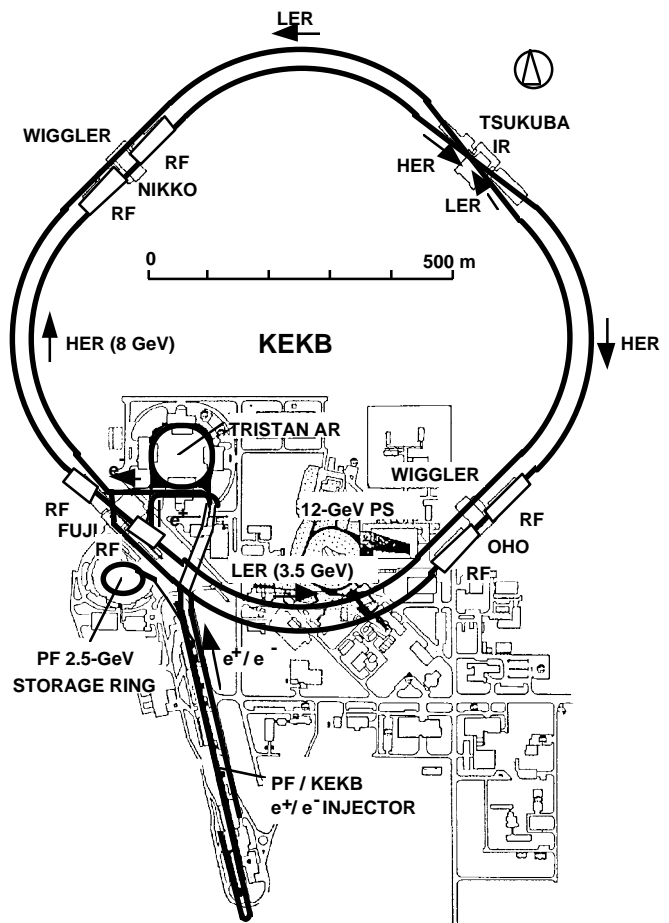
Fig.1 Schematic plan-view of KEKB.
