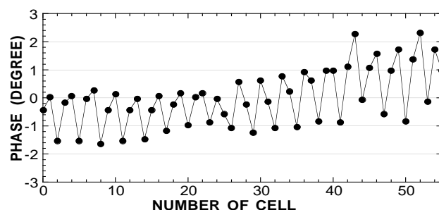
Fig. 6 Typical results of a nodal shift measurement: the standard deviation of phase error is about 0.9 degrees; the 2-m accelerator structures were fabricated by a "electroplating method" without any dimpling after machining.
