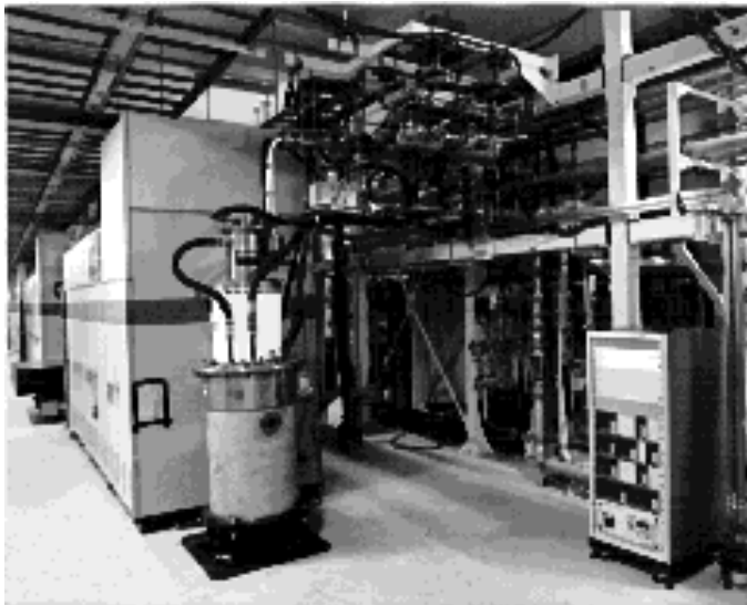
Fig.3 RF-source upgrade of the existing linac for KEKB: the modulator powers were doubled; the PFN cabinets became tall-boy in order to make a capacitance doubling; and the klystron outputs were upgraded from 30 MW to 50 MW while maintaining the height.
