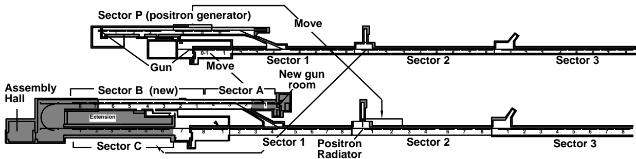
Fig. 2 Linac reconstruction from 2.5 GeV (upper) to 8 GeV (lower). The existing linac has 40 accelerator units which are divided into 5 sectors. The shadow areas are extension buildings to increase the number of accelerator units from 40 to 57.
