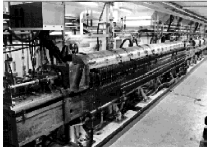
Fig.4 Positron generator replacement at a high-energy point of the upgraded linac. The accelerator structures behind the positron production target were improved in order to reduce the coupler field.
