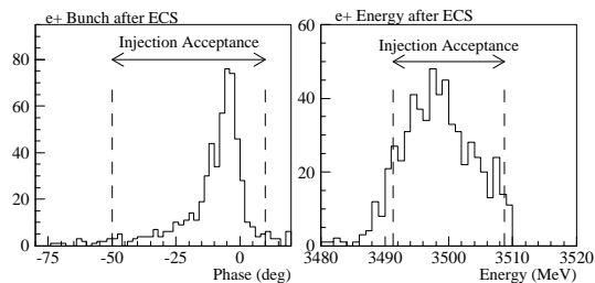
Fig. 7 Estimated bunch/energy width of the positrons after ECS.
