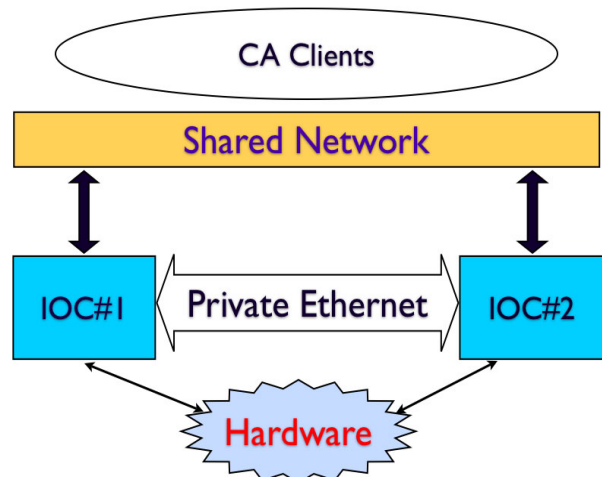
Figure 1: Hardware Architecture
